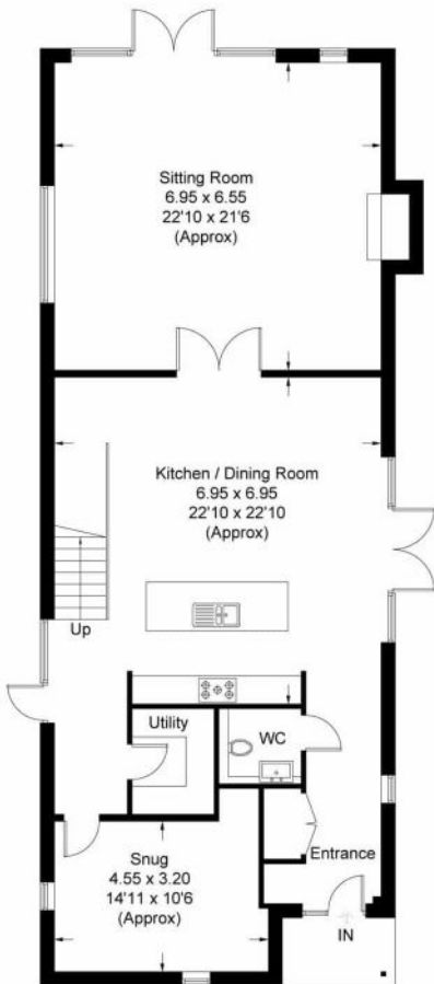
Ground Floor 133.6 sq m / 1438 sq ft
