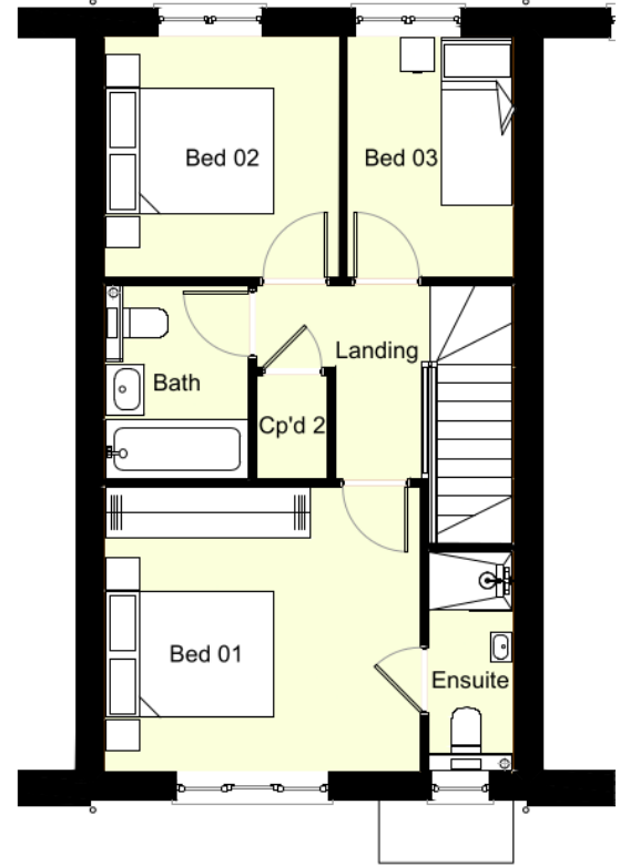
First Floor Layout Plots 02, 05 & 08 AS Plots 04, 06 & 07 Handed
