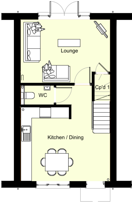
Ground Floor Layout Plots 02, 05 & 08 AS Plots 04, 06 & 07 Handed
